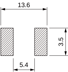
Land Pattern: [mm]
